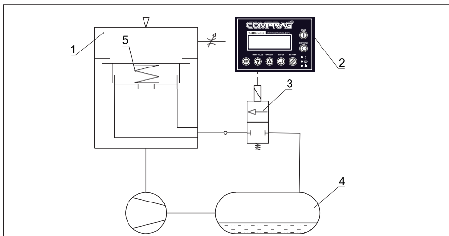
Fig. 2.5 Regulating system
